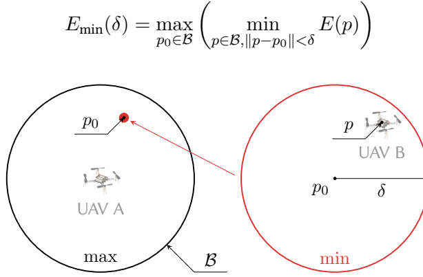
Figure 7: Maximum minimal achievable error for the space \mathcal{B} around the UAV
